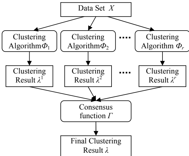
Figure 3. Basic Cluster Ensemble Framework
