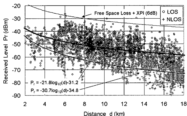
図 17 受信レベル距離特性 (送信局: Egezan) Fig. 17 Received level characteristics (Egezan).
