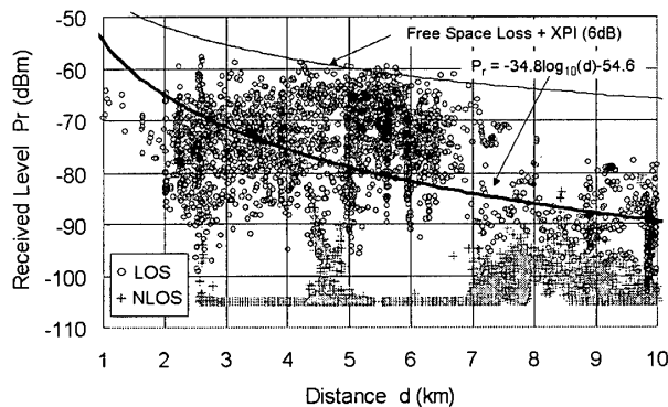
図 15 受信レベル距離特性 (送信局: Sato) Fig. 15 Received level characteristics (Sato).
