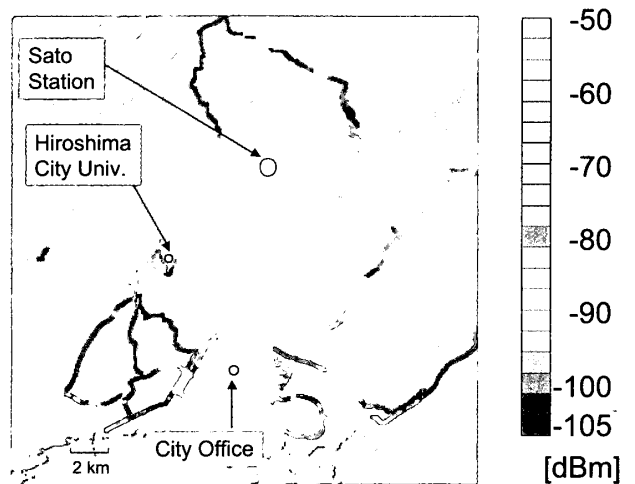
図 10 NLOS 受信レベルマップ (送信局 : Sato) Fig. 10 Received level map in NLOS area of the Sato station.
